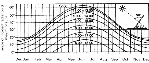
2 Incident radiation angle \beta (height of sun at the geographical latitude 50°N at various times, over the course of a year)
